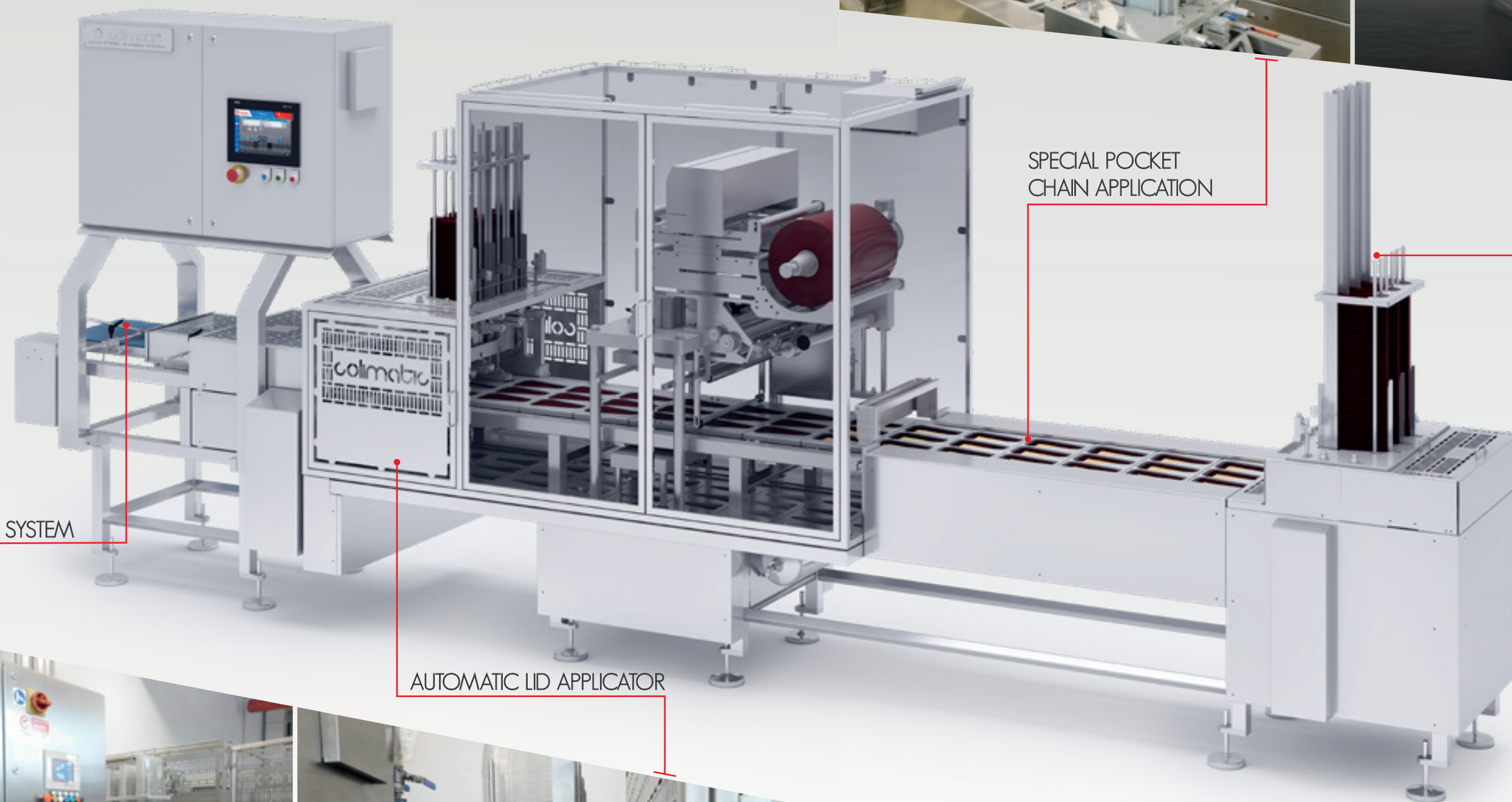
THERMOSEALING LINE MOD. TDF1500
