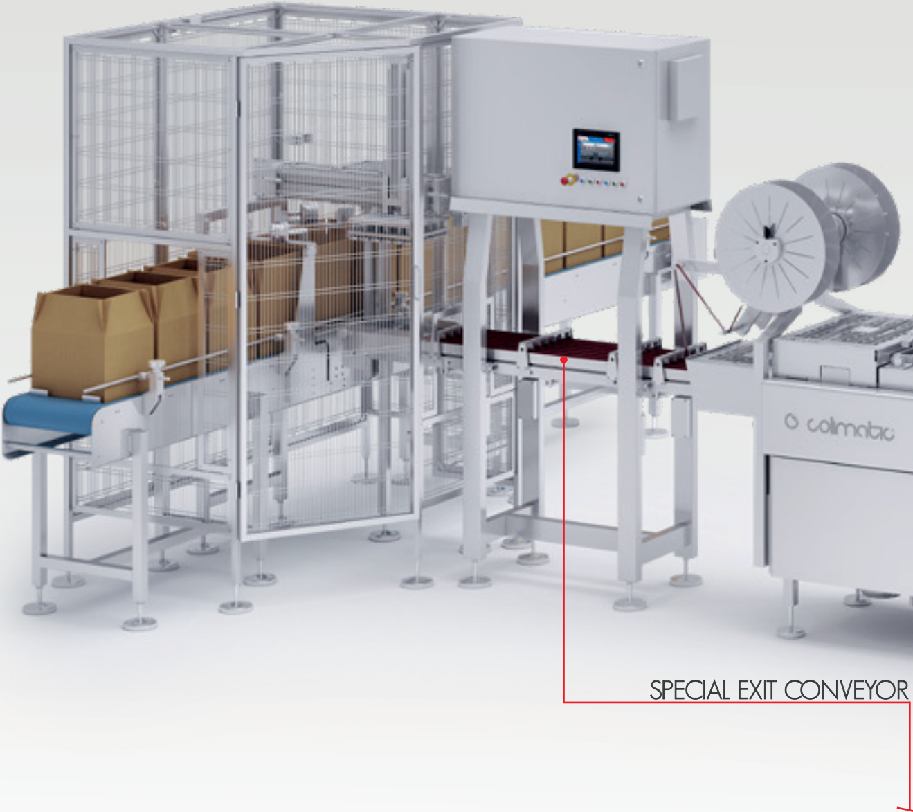
CARTONING LINE
